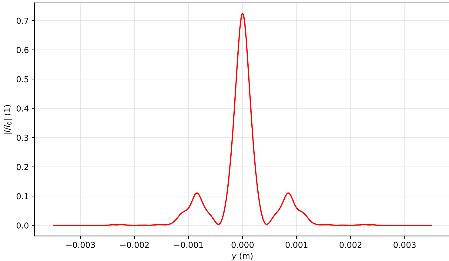
Intensity profile I(x=0, y, z=1.672)/I_0 , P_{in}=9.0P_{cr} , artificial time
